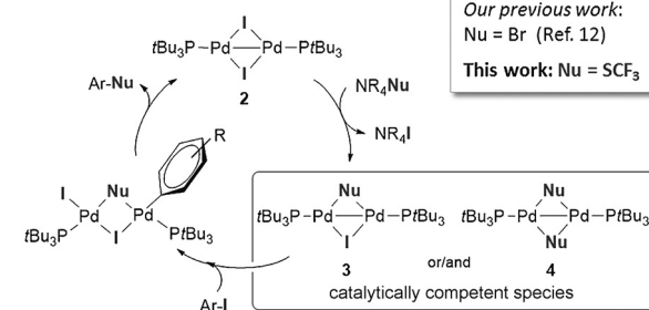
Figure 1. Pd I -dimer catalysis concept (bottom).
